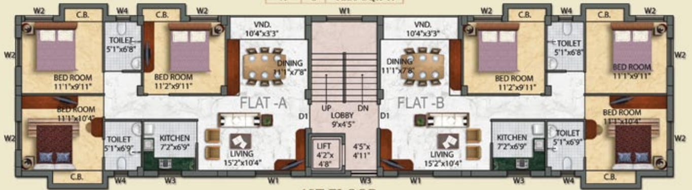
1ST FLOOR
